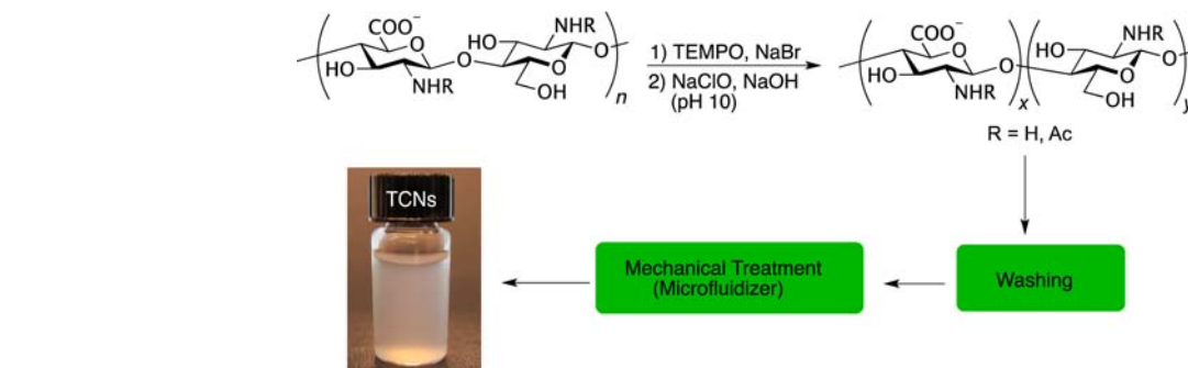
Scheme 1. Chitin Nanocrystal Formation via TEMPO-Mediated Oxidation of Chitin
