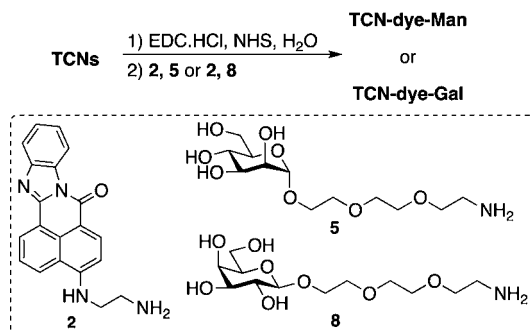
Scheme 2. Synthesis of Dually Functionalized TCNs
